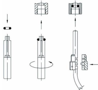
Abb. 10: Montage Adapterset
